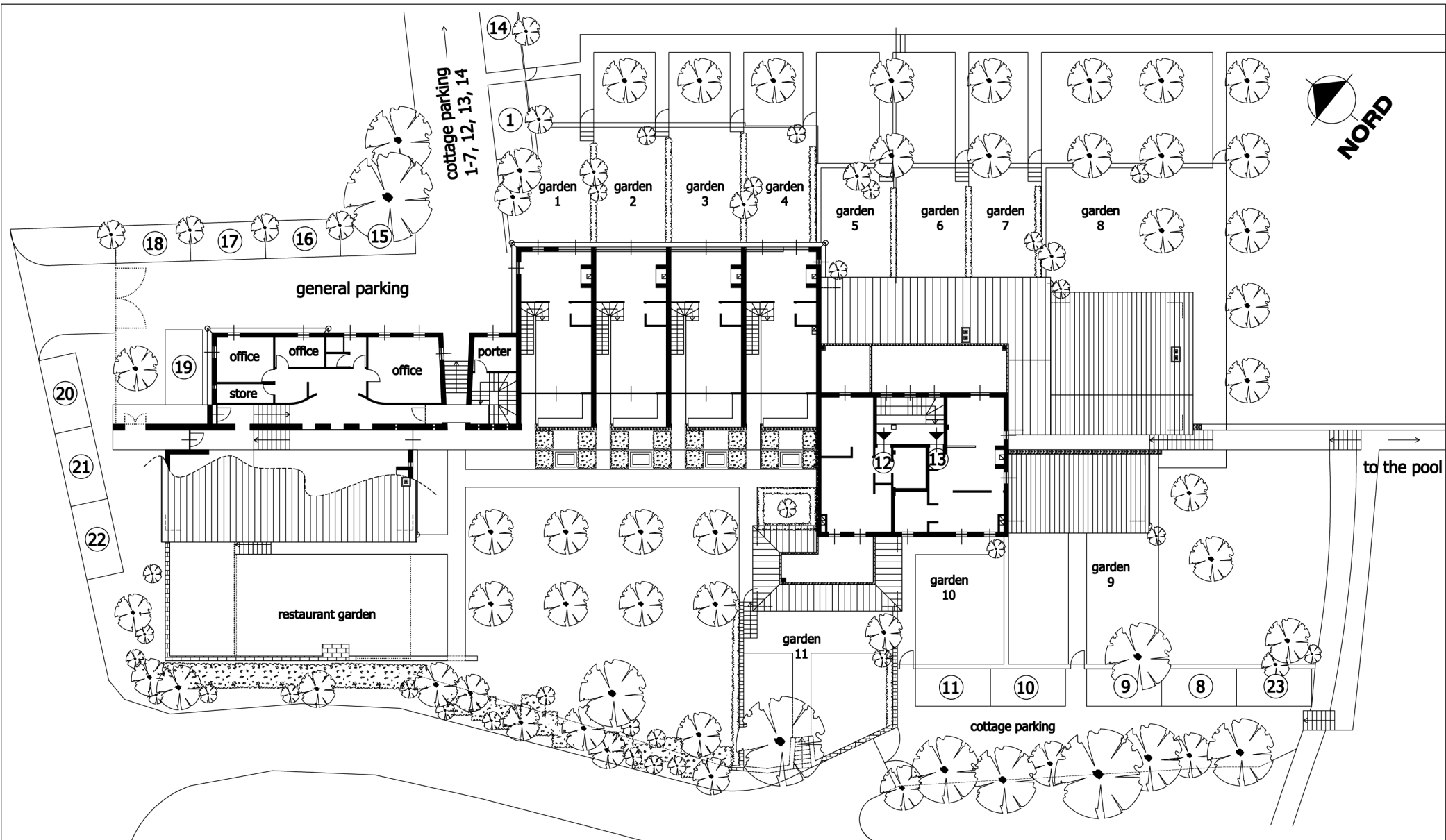
Borgo69 - First Floor Plan
