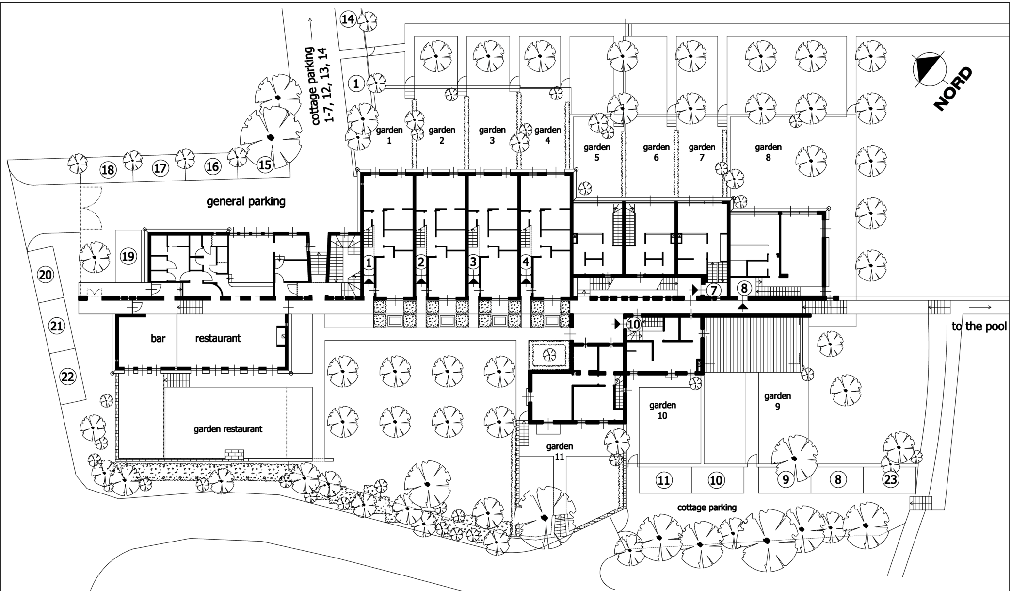
Borgo69 - Ground Floor Plan
